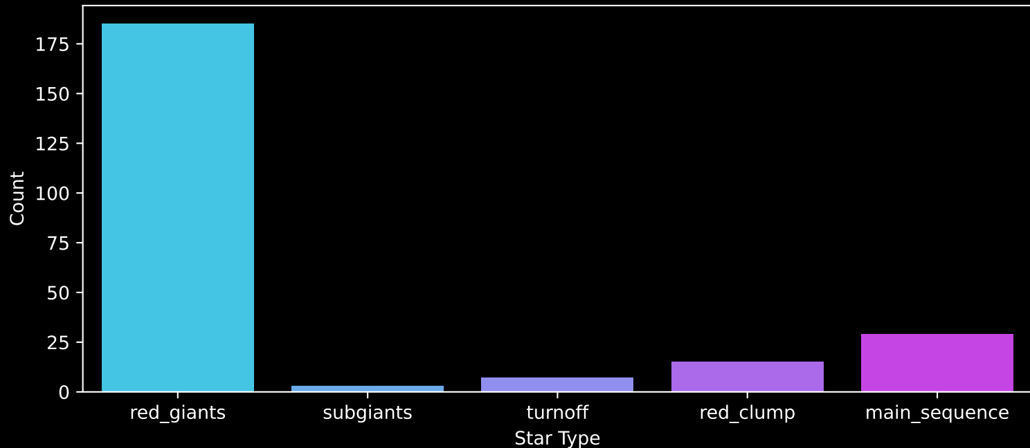
APOGEE DR17 Field: [296-12] Count plot of Star Type
