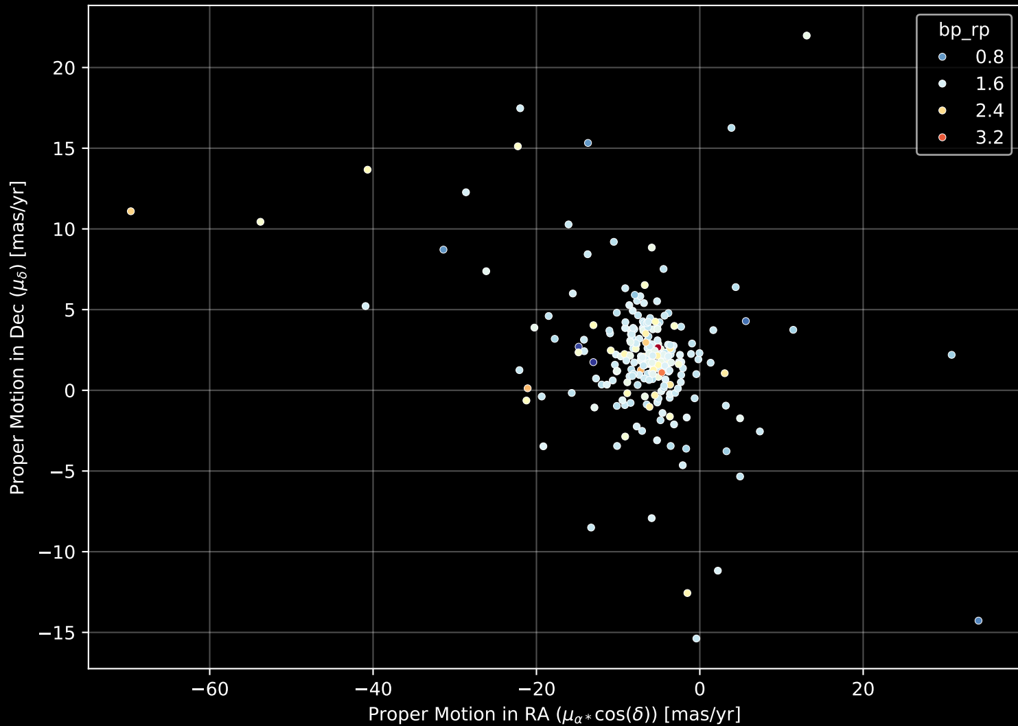
APOGEE DR17 Field: [296-12] Proper Motion Diagram (n= 239)
