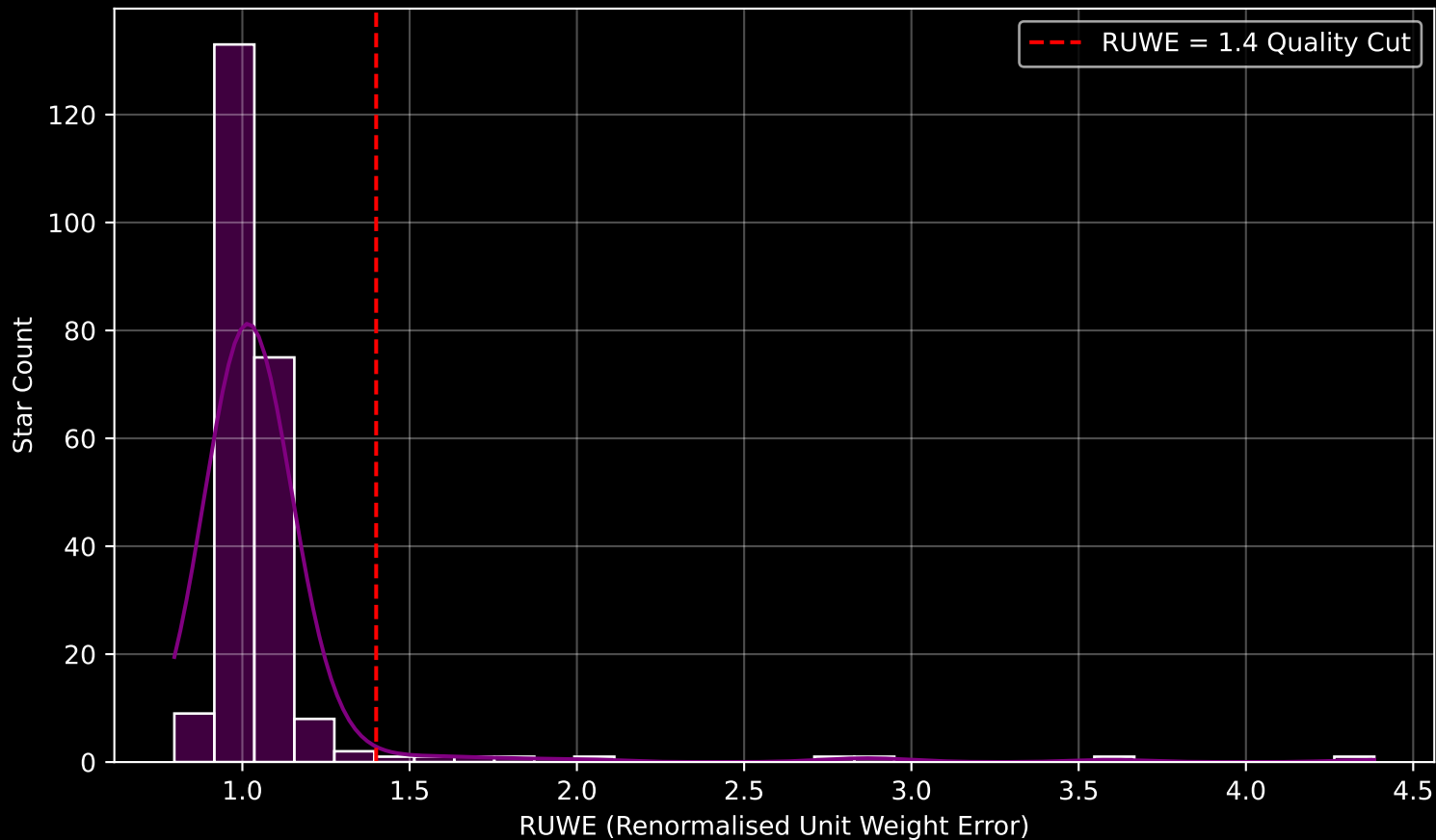
GAPOGEE DR17 Field [296-12] RUWE Distribution (n= 236)
