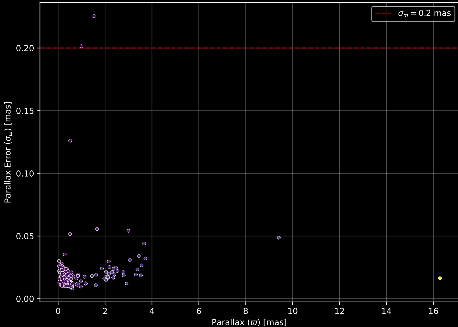
APOGEE DR17 Field: [296-12] Parallax Quality (n= 239)
