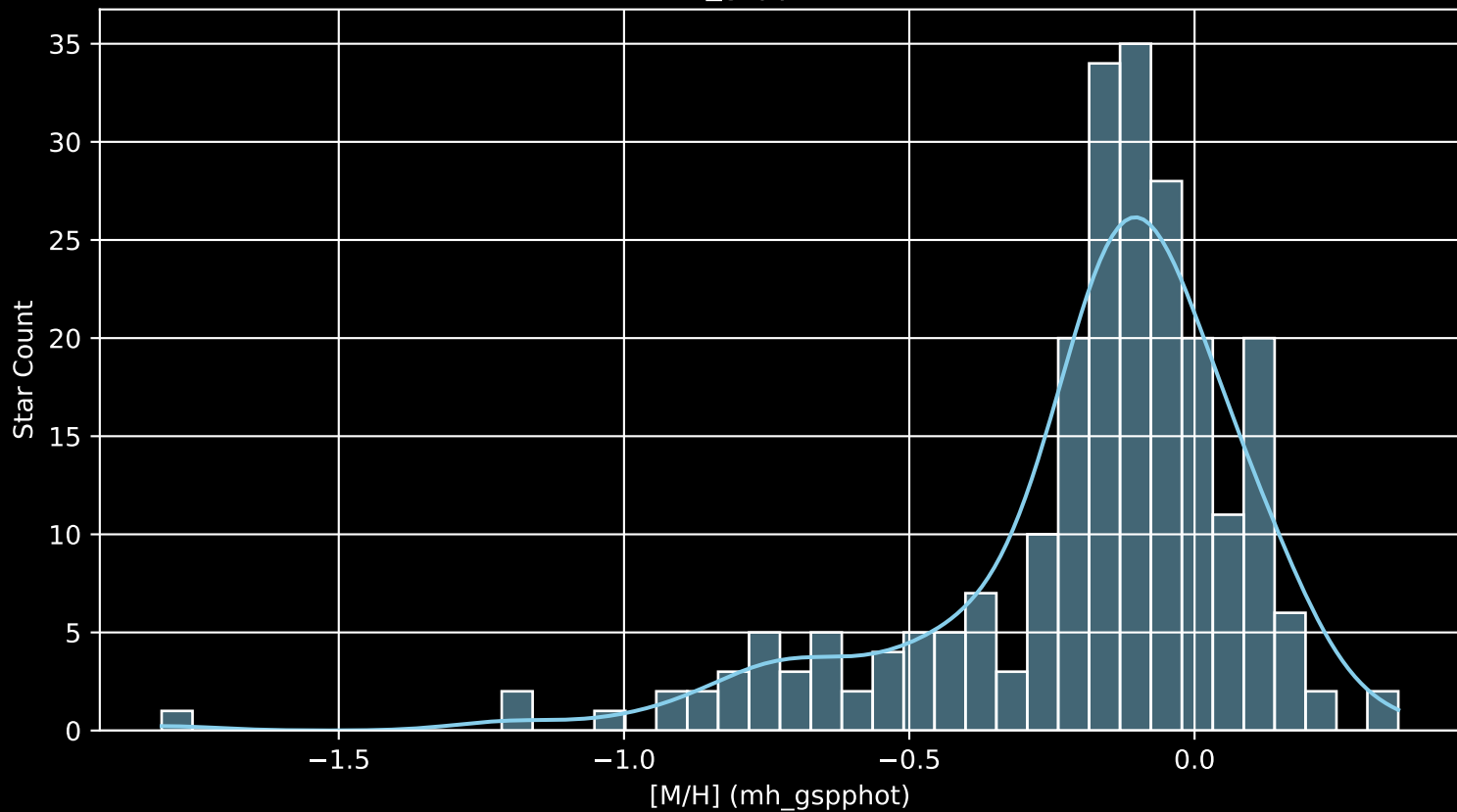
APOGEE DR17 Field: [296-12 [M/H] (mh_gspphot) (n= 238)
