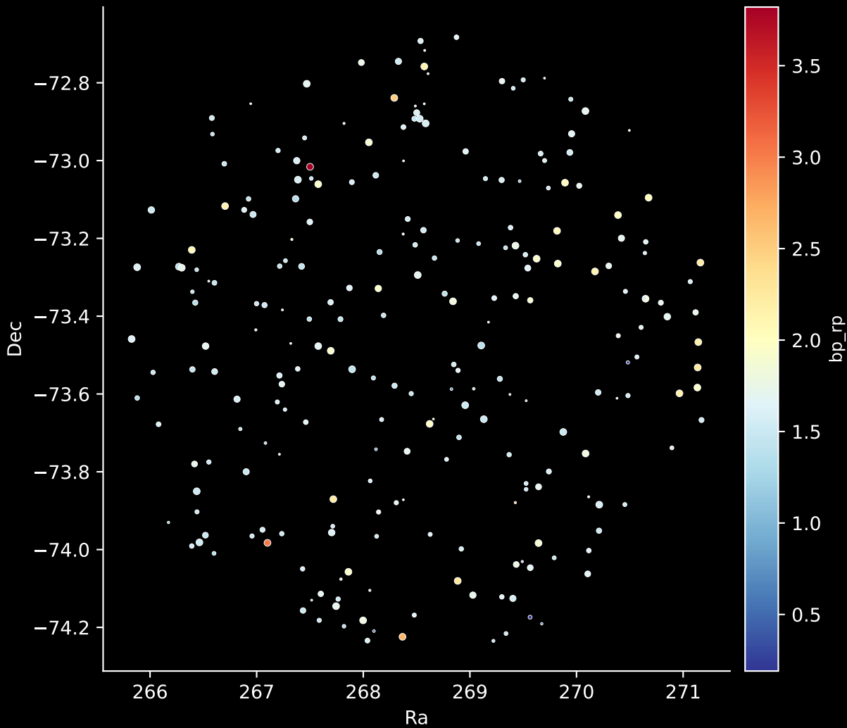
APOGEE DR17 Field: [296-12] Stars: 239
