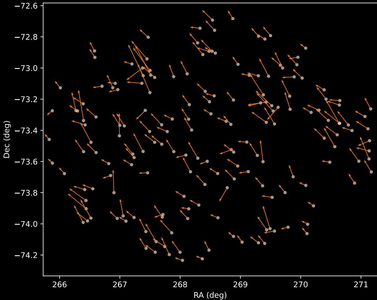
APOGEE DR17 Cluster 2 Proper Motion Vectors (n=178)
